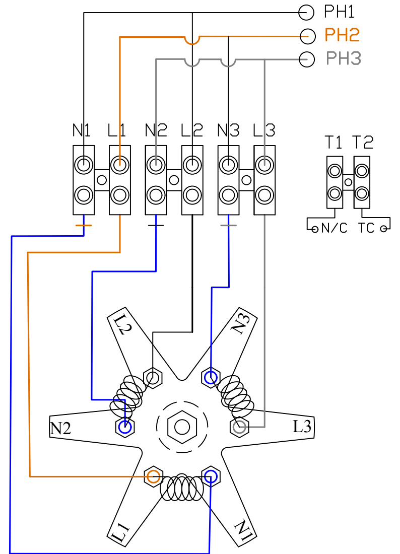
3-PHASE (DELTA) 415v
