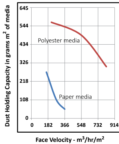
Face Velocity vs. Dust Holding Capacity
