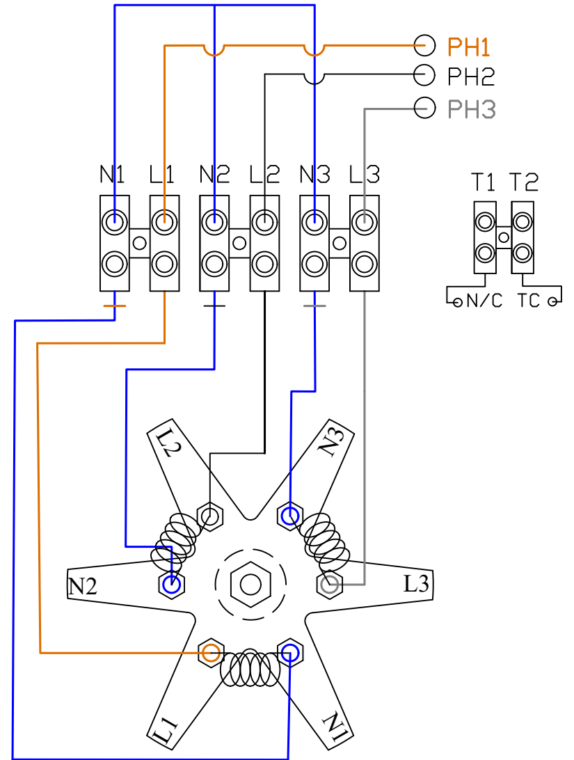
3-PHASE 3 WIRE CONNECTION 415vac
